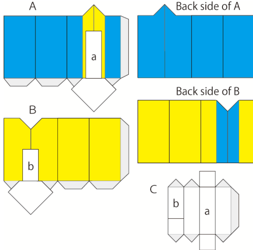
Figure A.1: Unfolded surfaces of the components of the object shown in Fig. 1.
